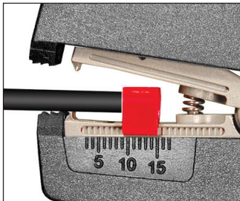
Wire Stop for precise strip length
