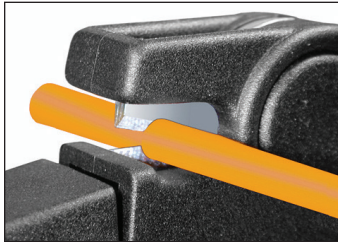
Wire Cutter with safety guard
